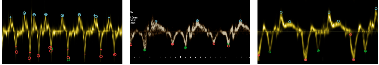
Fig. 3: Examples of incorrect patient-level predictions. The ground truths (+) and predictions (o) of tissue velocity peaks S' (cyan), e' (red), and a' (green) are overlaid on the input image. Left: Unusual signal in which no a' waves are preset. The model confuses a' and e' and misses two S' waves (false . Centre: The last a' wave is marked as a' and e' (false positive). Right: There are two S' waves marked in two of the waveforms and two e' waves marked in the last waveform.
